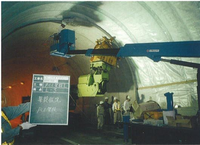
● PCL版据付状況-1
